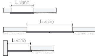
VISTA IN PANTA
